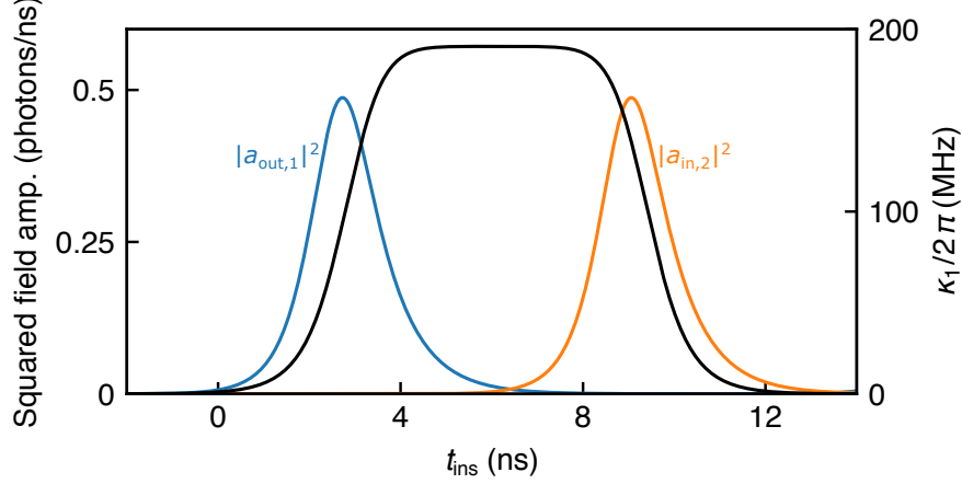
Figure S6. Traveling photon envelope estimated from simulations. The horizontal axis is the instantaneous time t_{\text{ins}} of the dynamic evolution, calculated for a control pulse width set to t = 12.2 ns for optimized state transfer. The blue curve shows the emitted photon envelope |a_{\text{out},1}|^2 ; the orange curve shows the captured photon envelope |a_{\text{in},2}|^2 . The black curve (right axis) shows the decay rate \kappa_1/2\pi for qubit Q_1 ; qubit Q_2 is very similar.
