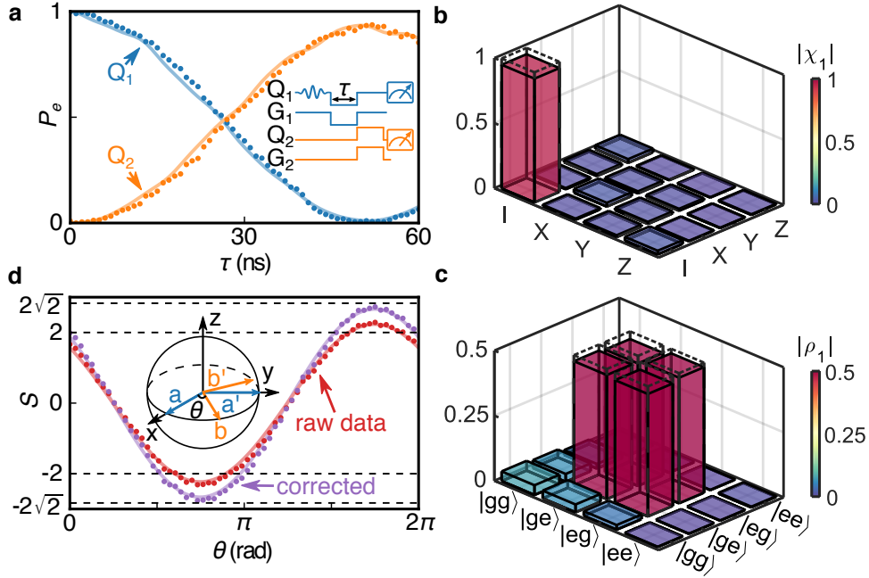
Figure 2. State transfer, remote entanglement, and Bell violation using the relay method. a , Quantum state transfer from Q_1 to Q_2 using the n = 73 , \omega_n/2\pi = 5.744 GHz standing mode as a relay, showing the |e\rangle state probability P_e for each qubit versus swap time \tau . Solid lines: Numerical simulations. Inset: Control pulse sequence. b , Process matrix (absolute values shown as colored bars) of the state transfer process with a fidelity \mathcal{F}_1^p = 0.952 \pm 0.009 . Dashed-outline frames: Ideal process matrix. c , Bell state density matrix (absolute values shown as colored bars), with a state fidelity \mathcal{F}_1^s = 0.950 \pm 0.005 . Dashed-outline frames: Ideal density matrix. d , Bell test, showing CHSH correlation S versus measurement angle \theta . Red dots: No measurement correction; purple dots: With measurement correction. Solid lines: Numerical simulations using \rho_1 from panel c. The classical and quantum limits are marked with horizontal dashed lines. Inset: Measurement axes a, a', b, b' on Bloch sphere.
