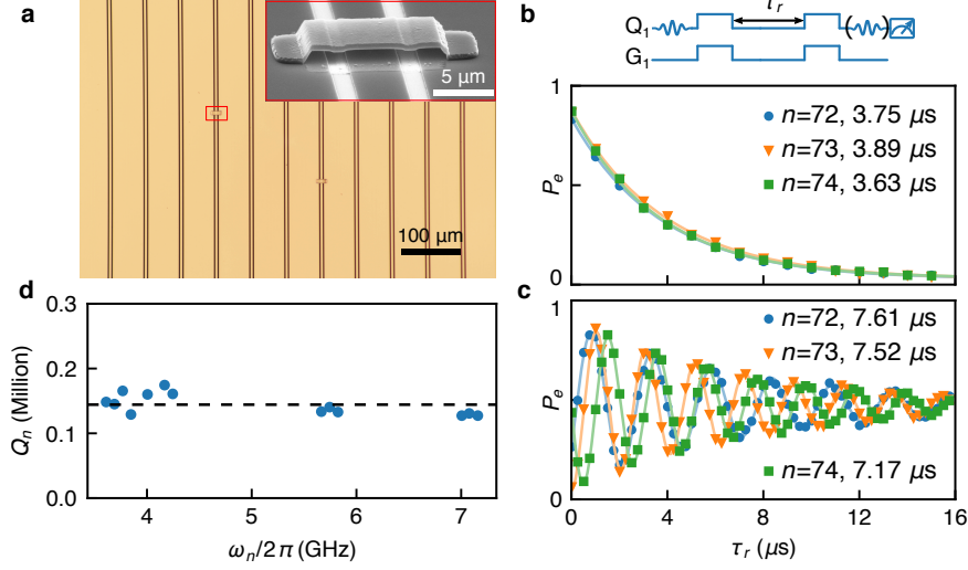
Figure S3. Transmission line characterization. a , Optical micrograph of a small portion of the transmission line, which has a 4 \mu\text{m} wide center trace and a 2 \mu\text{m} gap to the ground plane on either side. The transmission line meanders are separated by 60 \mu\text{m} , and the line has 390 air-bridge crossovers evenly distributed along the line every 2 \text{mm} , suppressing unwanted slot-line modes and other microwave resonances. Inset: Scanning electron micrograph picture of an air-bridge crossover. b , c , The lifetime T_{1n} and Ramsey dephasing time T_{2n} of three of the six resonant modes shown in Fig. 1d. We find T_{2n} \approx 2T_{1n} , indicating negligible dephasing noise in the transmission line. Solid lines: Fits to each mode's data. Top: Control pulse sequence. d , Quality factor Q_n = \omega_n T_{1n} measured for different modes from 3.6 \text{GHz} to 7.2 \text{GHz} . We find that the quality factor is more or less constant over this frequency range, with an average \langle Q \rangle \sim 1.44 \times 10^5 as indicated by the horizontal dashed line.
