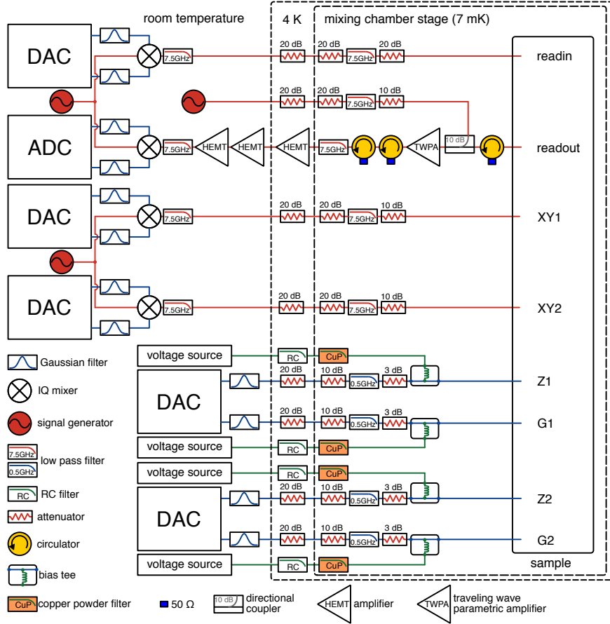
Figure S1. Electronics and wiring. Red lines correspond to radiofrequency (RF) and microwave signals for qubit XY control and measurement, blue lines correspond to intermediate frequency (IF) signals for fast qubit Z or coupler control, and green lines correspond to quasi-DC signals for steady qubit Z or coupler bias offset. The IF and DC signals for each bias channel are combined using a custom-made cryogenic bias tee mounted at the mixing chamber stage.
