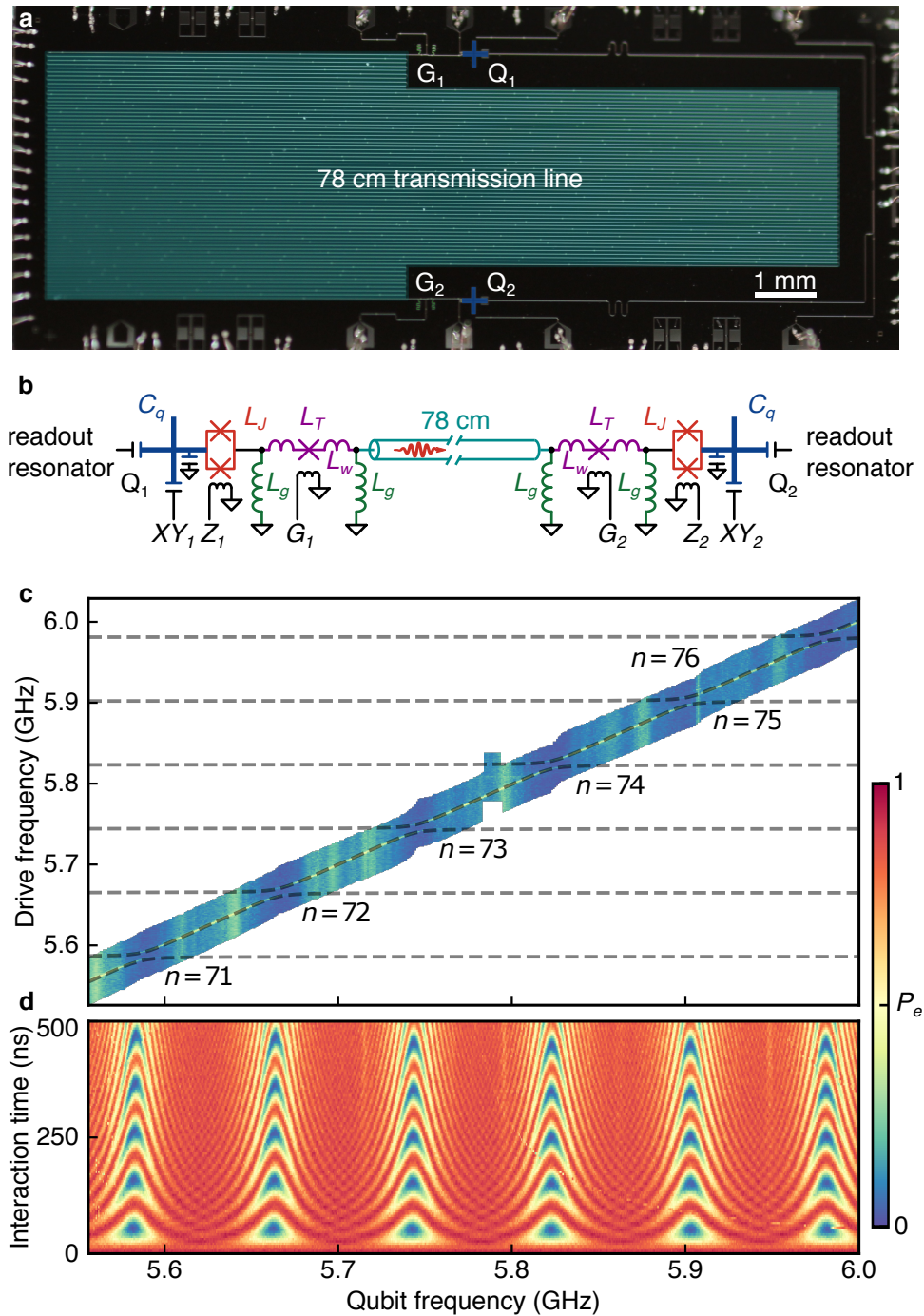
Figure 1. Device description. a , Photograph of device, showing two qubits Q_1 and Q_2 (blue) connected via tunable couplers G_1 and G_2 (green) to a 78 cm-long coplanar transmission line (cyan). b , Circuit schematic, with parameters listed in Table S2 (Supplementary Information). c , Spectroscopy of qubit Q_1 interacting with six transmission line standing modes. Black dashed lines: Numerical simulations. d , Vacuum Rabi swaps between Q_1 and the six standing modes. The coupling is set to g_1/2\pi = 5 MHz \ll \omega_{\text{FSR}}/2\pi .
