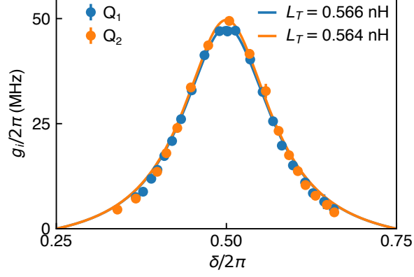
Figure S4. Coupling strength versus coupler junction phase \delta . We measure the qubit spectrum at different coupler bias values, similar to Fig. 3a, and fit the spectrum to obtain the coupling strength g_i . The maximum coupling is about 47 MHz for Q_1 and 49 MHz for Q_2 . Error bars are one standard deviation.
