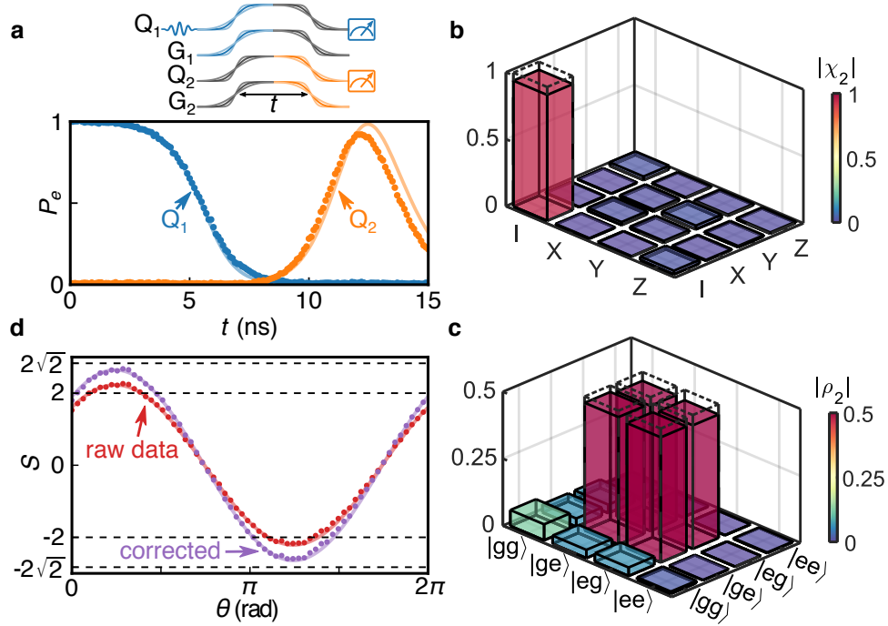
Figure 4. State transfer, remote entanglement and Bell violation using itinerant photons. a , Using optimized control pulses for the couplers while keeping the qubit frequency fixed, we achieve a high-fidelity state transfer, with a maximum transfer probability of 0.919 \pm 0.004 in 12.2 ns. Solid lines: Numerical simulations. Top: Control pulse sequence. The rising edge of Q_1 's control pulse determines the emission process, and the falling edge of Q_2 's control pulse determines the capture process. b , Quantum process tomography, with a process fidelity \mathcal{F}_2^p = 0.940 \pm 0.008 . Dashed-outline frames: Ideal process matrix. c , Density matrix of the Bell state generated by sending half an itinerant photon from Q_1 to Q_2 , with a state fidelity \mathcal{F}_2^s = 0.936 \pm 0.006 and a concurrence \mathcal{C}_2 = 0.914 \pm 0.014 . Dashed-outline frames: Ideal density matrix. d , Bell test, showing the CHSH correlation S versus measurement angle \theta . Red dots: No measurement correction; purple dots: With measurement correction. Solid lines: Numerical simulations using \rho_2 from panel c . The correlation is maximized at \theta = 0.84 rad, where S = 2.223 \pm 0.023 without measurement correction. Classical and quantum limits are marked with horizontal dashed lines.
