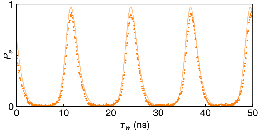
Figure S7. Optimized itinerant photon catch process for qubit Q_2 , analogous to Fig. 3d in the main text with a slight adjustment to the control pulse optimization. The capture probability is found to be 0.917 \pm 0.006 . Solid line is simulation.
